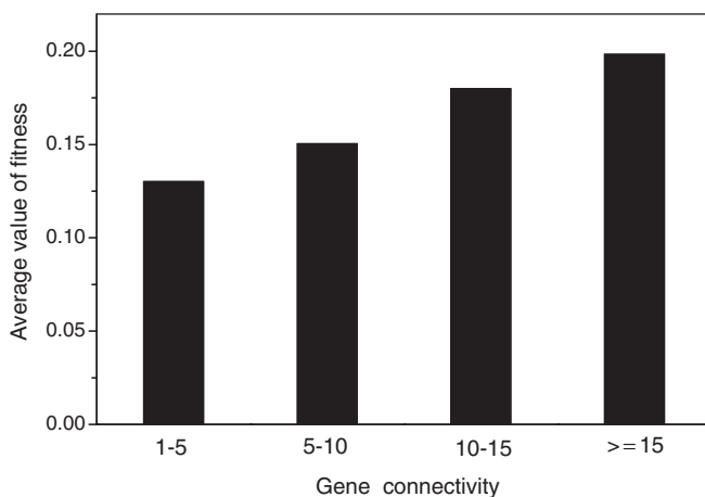
Fig. 3. The fitness (indispensability) of 132 query genes in yeast S.cerevisiae versus gene connectivity in the genetic interaction network determined through the SGA analysis. Gene connectivity is measured by the node degree (number of interactions) in the network.
