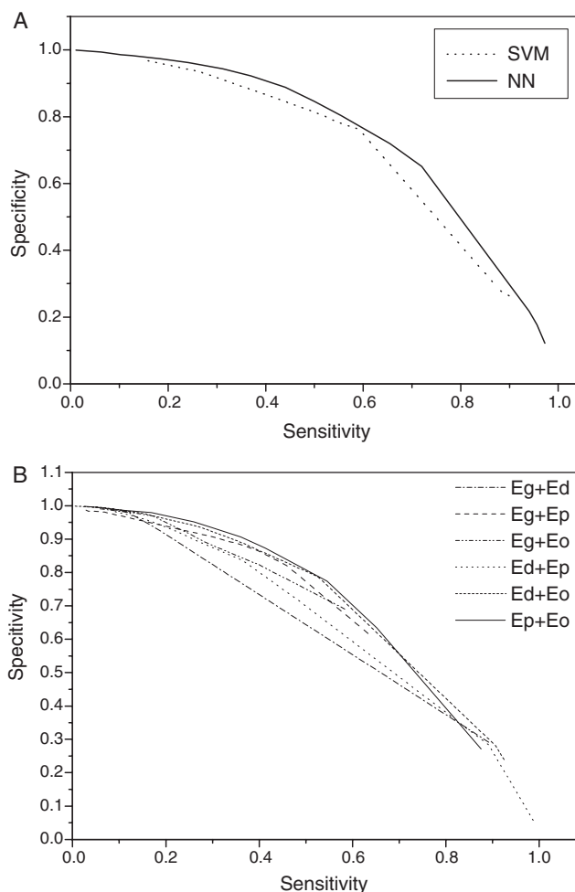
Fig. 2. ROC curves of protein dispensability predictions. (A) Sensitivity and specificity of neural network (NN) and SVM. (B) Sensitivity and specificity of neural network for different feature combinations (e.g. connectivity of gene-expression data; E_d , gene duplication data; E_p , protein connectivity in protein-interaction network; and E_o , gene conservation rate).
